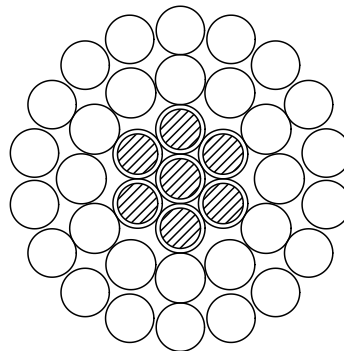
ACSR/AC 120, 160, 200, 240 (AL30, AC7)
