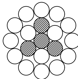
S-ACSR 62, 80, 100, 120 (AL15, St4)
