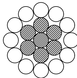
IACSR 64, 79, 97, 120, 150 (AL12, St7)
