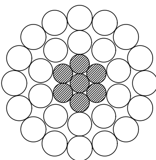
ACSR 330, 410 (AL26, St7)
